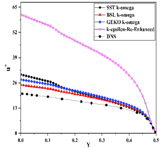
Figure 3. Dimensionless velocity obtained from DNS and RANS results on the buoyancy-opposing side for Ri = 0.25
