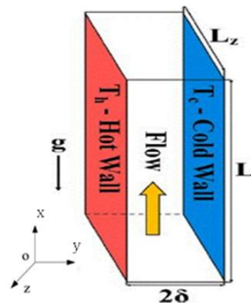
Figure 1. Coordinate system and flow geometry.
