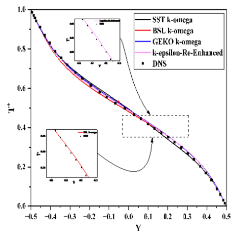
Figure 4. Dimensionless temperature obtained from DNS and RANS results across the entire flow domain for Ri = 0.25
