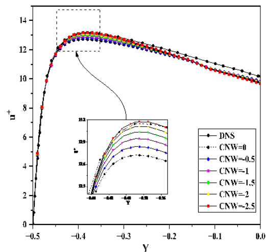
Figure 7. Dimensionless velocity obtained from DNS and GEKO results on the buoyancy-assisting side for Ri = 0.25 with different CNW values
