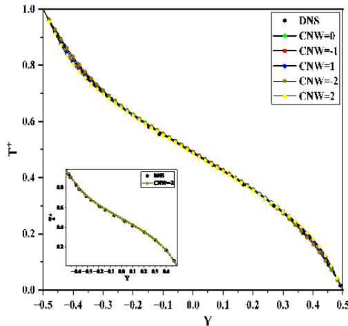
Figure 9. Dimensionless temperature obtained from DNS and RANS results across the entire flow domain for Ri = 0.25 with different CNW values
