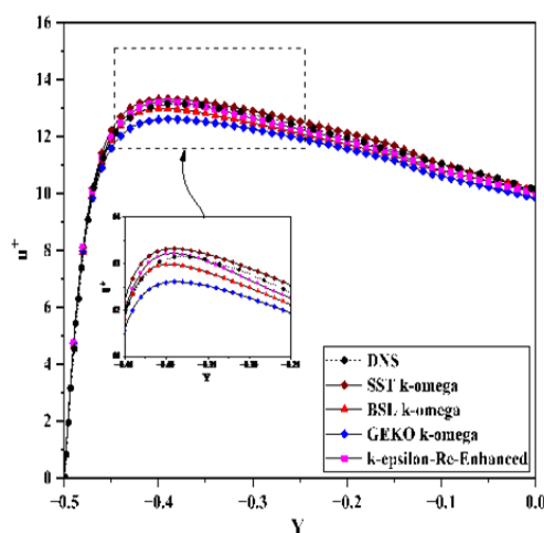
Figure 2. Dimensionless velocity obtained from DNS and RANS results on the buoyancy-assisting side for Ri = 0.25
