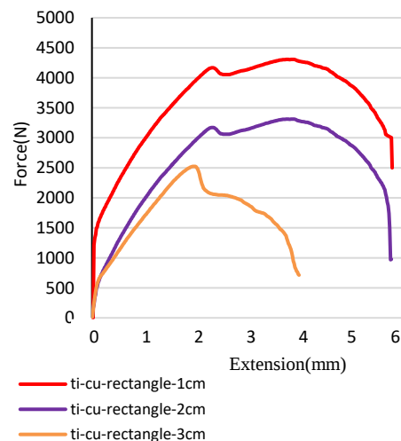
TI-CU-Rectangle patch
